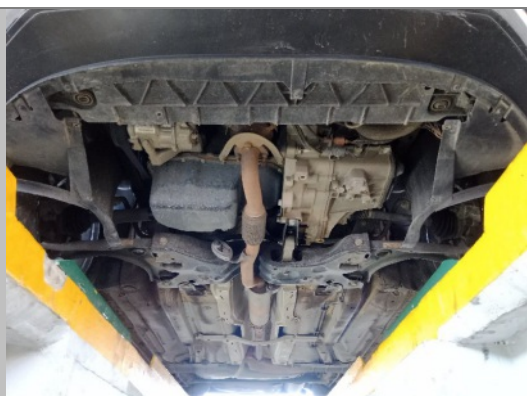
CHASSIS
